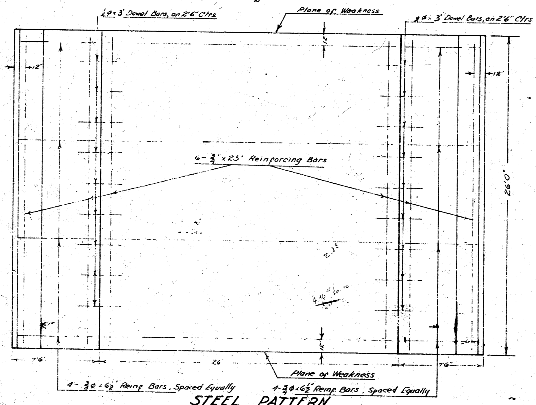
STEEL PATTERN
