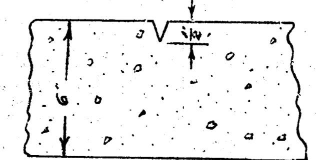
Detail Plane of Weakness Plane of Weakness to be cut with Double-Ridge Groover to Depth 4" Shown in a Straight Line from Curb to Curb 24" Ctr to Ctr.
