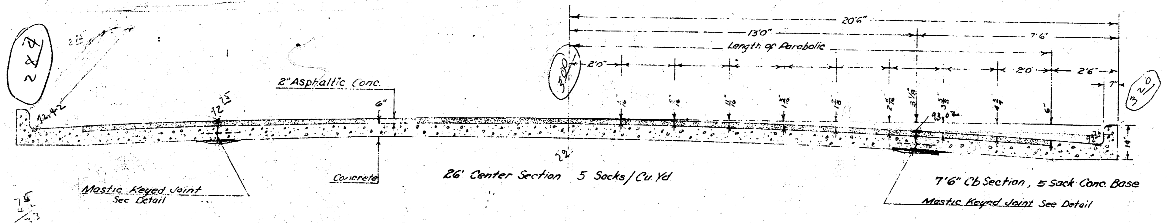
TYPICAL SECTION
