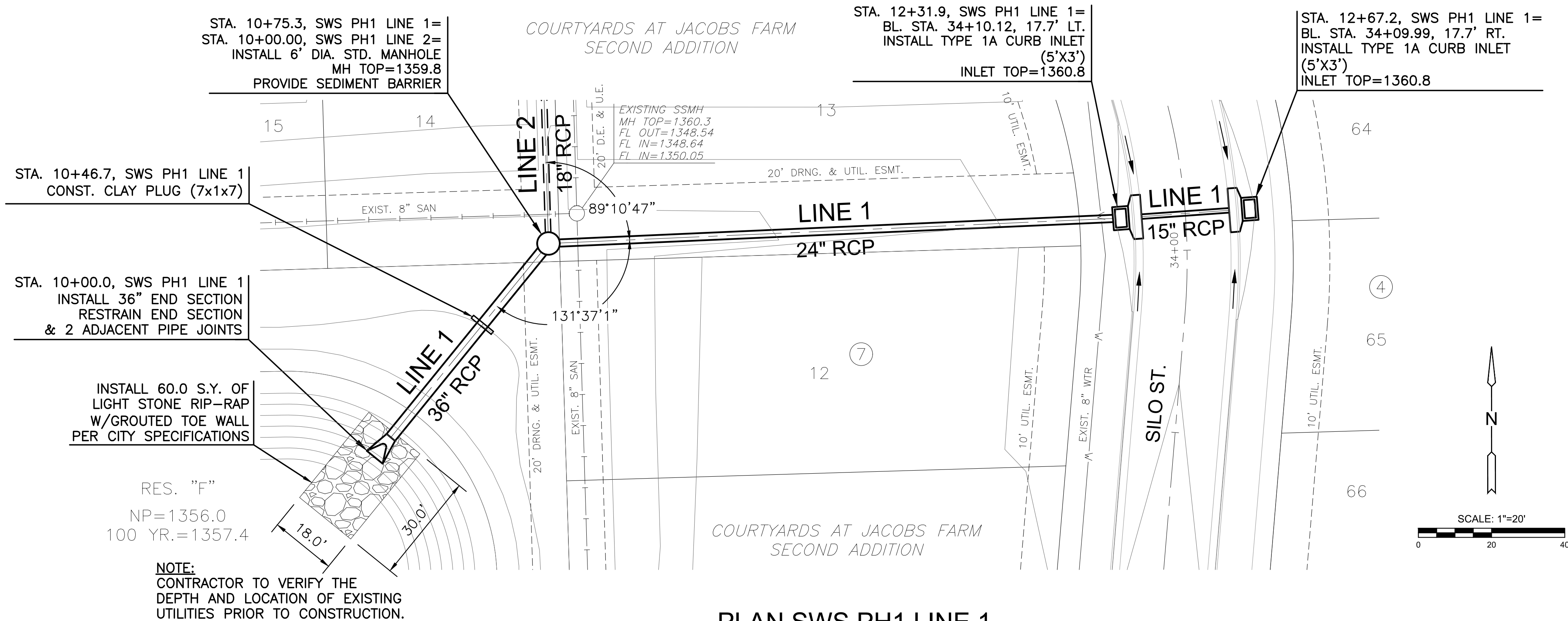
PLAN SWS PH1 LINE 1 PROFILE SWS PH1 LINE 1
