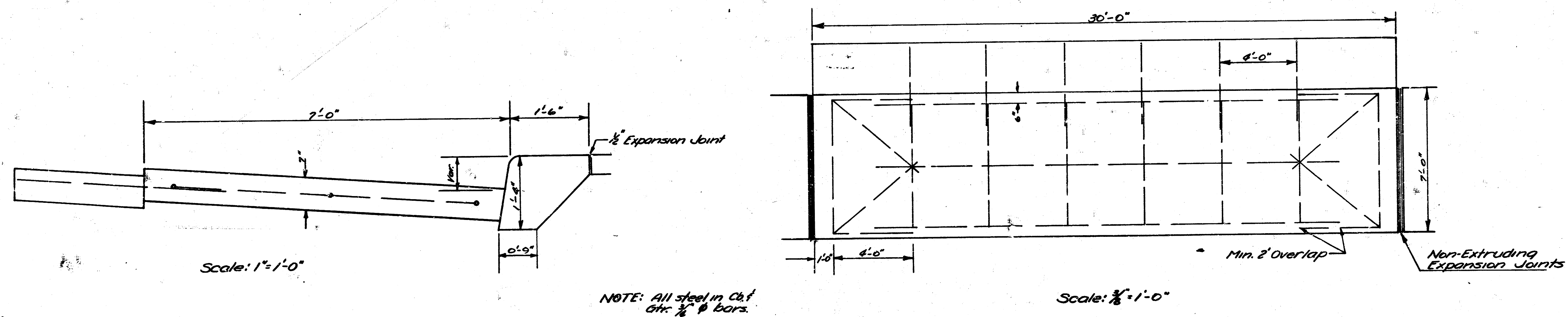
DETAILS of CURB & GUTTER
