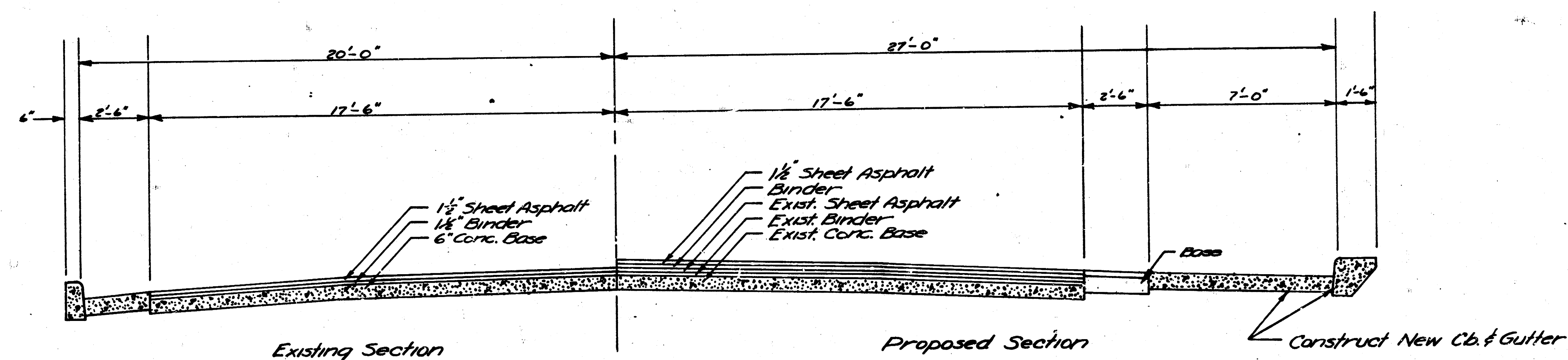
Scale: 3/8" = 1'-0" TYPICAL SECTION S.L. WATERMAN-N.L. LEWIS
