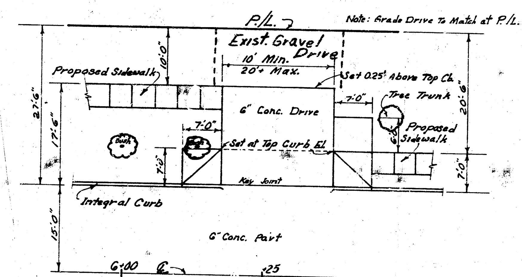
SPECIAL RAMP DRIVE DETAILS SCALE: 1" = 10'
