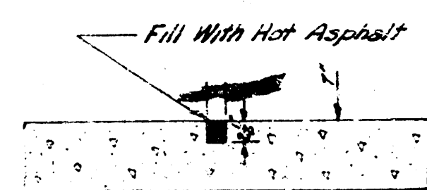
CONTRACTION JOINT DETAIL NO SCALE
