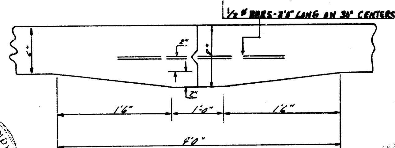
DETAIL OF MASTIC KEY JOINT NO SCALE
