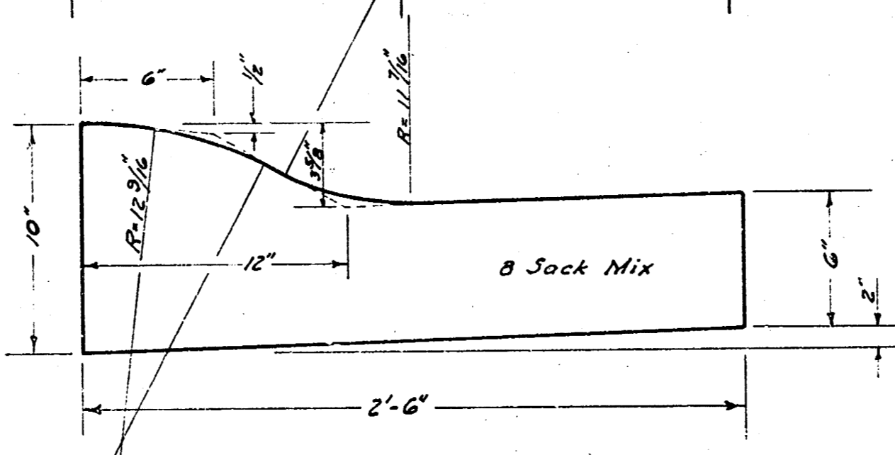
ROLL CURB & GUTTER DETAIL
