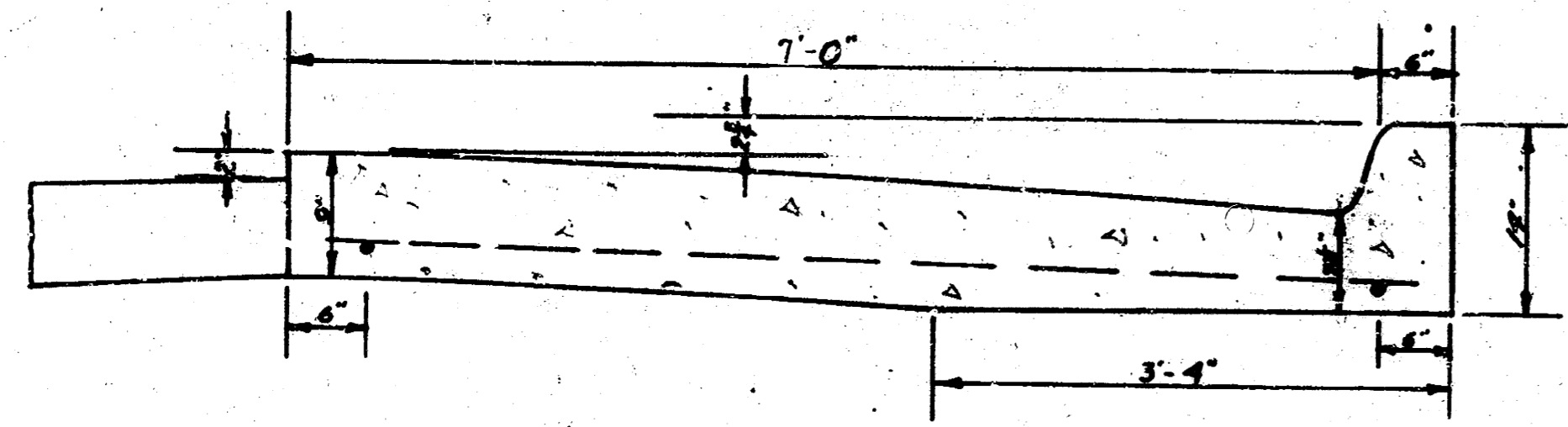
DETAIL OF 7" CURB & GUTTER SECTION Scale: 1"=1'-0"
