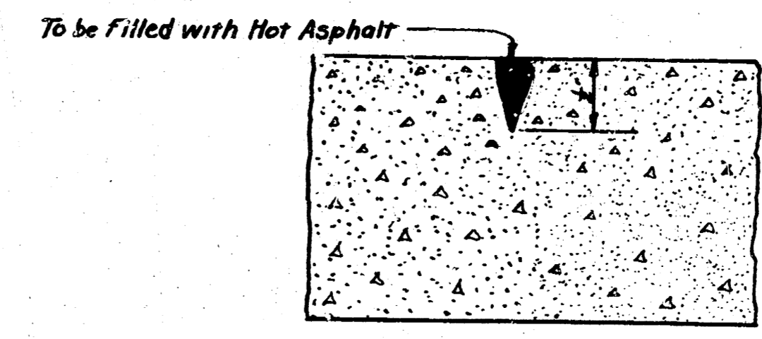
DETAIL OF PLANE OF WEARNESS EVERY 9th JOINT TO BE EXPANSION JOINT No Scale
