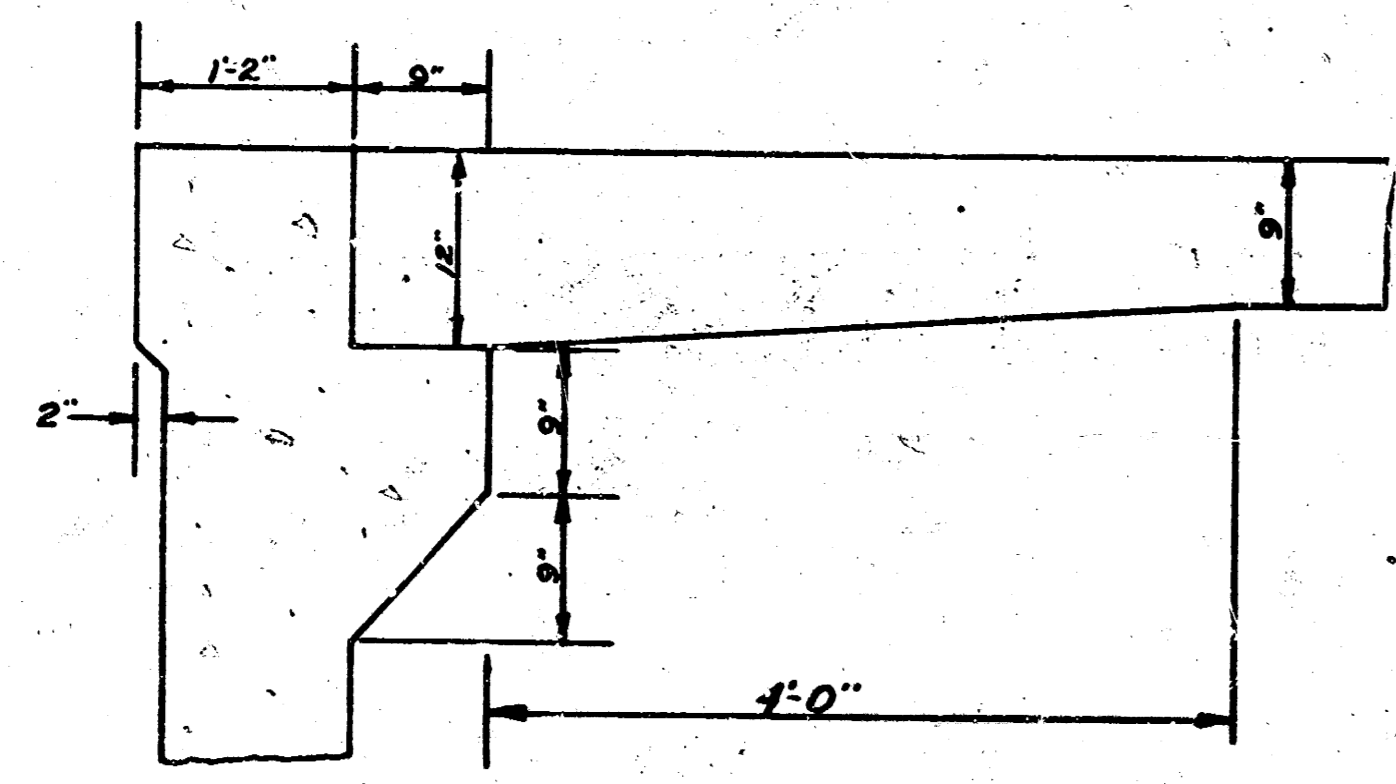
DETAIL OF TRANSITION FROM BRIDGE SEAT AT Scale: 1"=1'-0"
