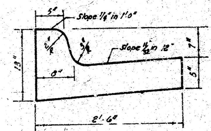
ROLL TYPE CURB & GUTTER
