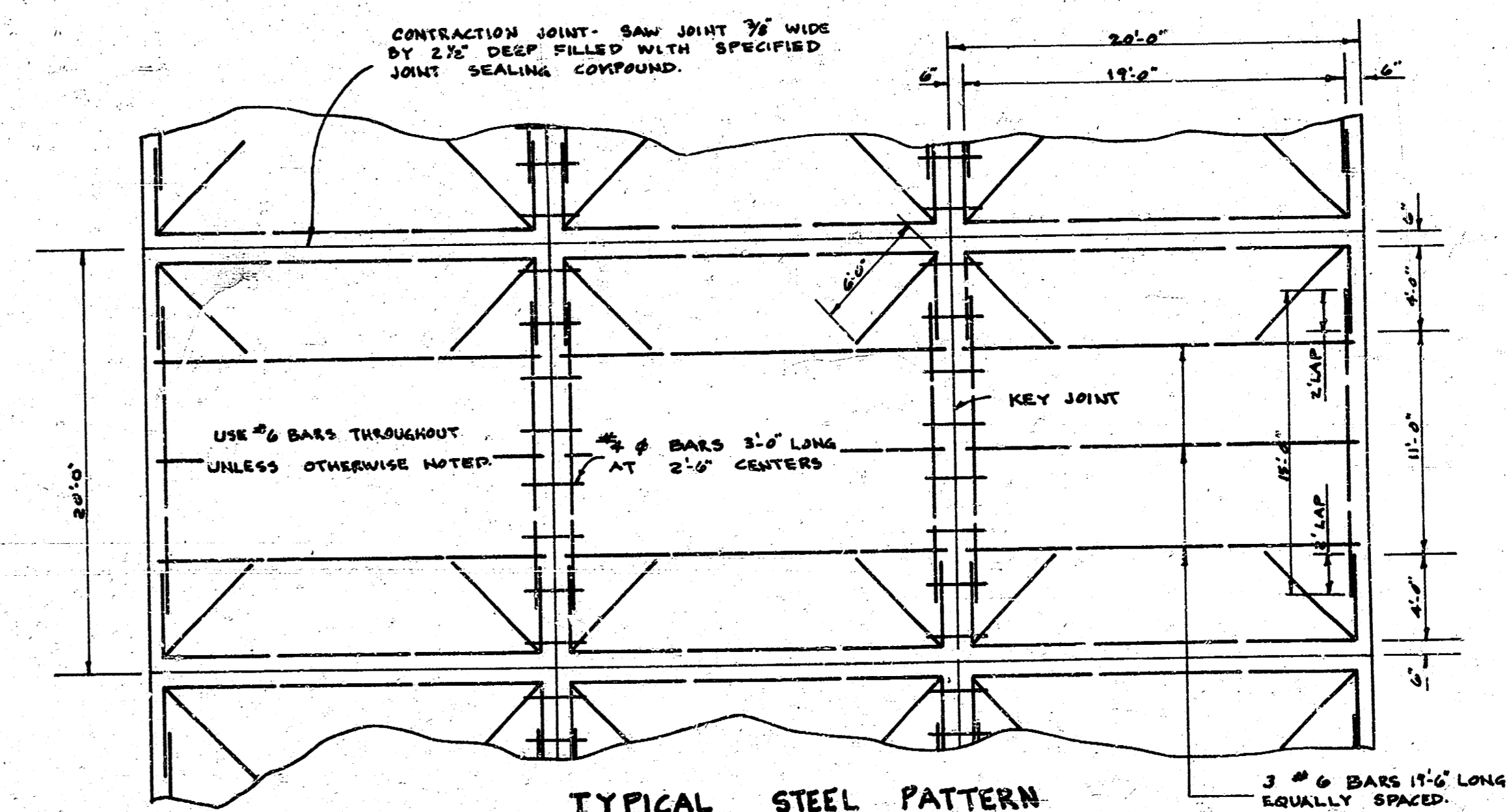
TYPICAL STEEL PATTERN SOUTH PARKING LOT
