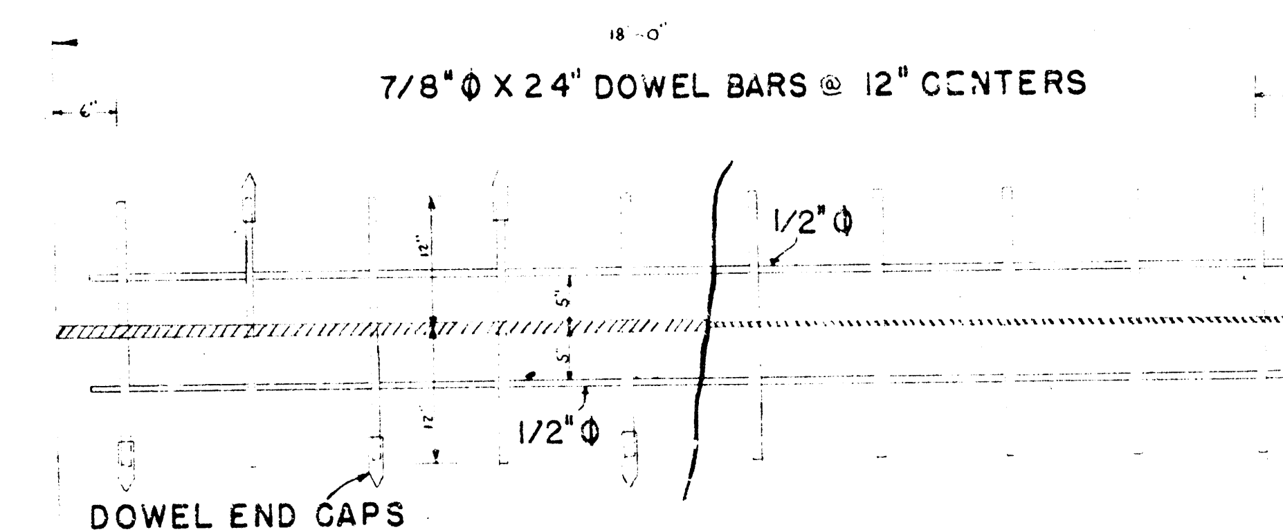
PART PLAN OF EXPANSION JOINT SCALE 1" = 1' PART PLAN OF CONTRACTION JOINT
