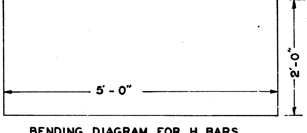
BENDING DIAGRAM FOR H BARS
