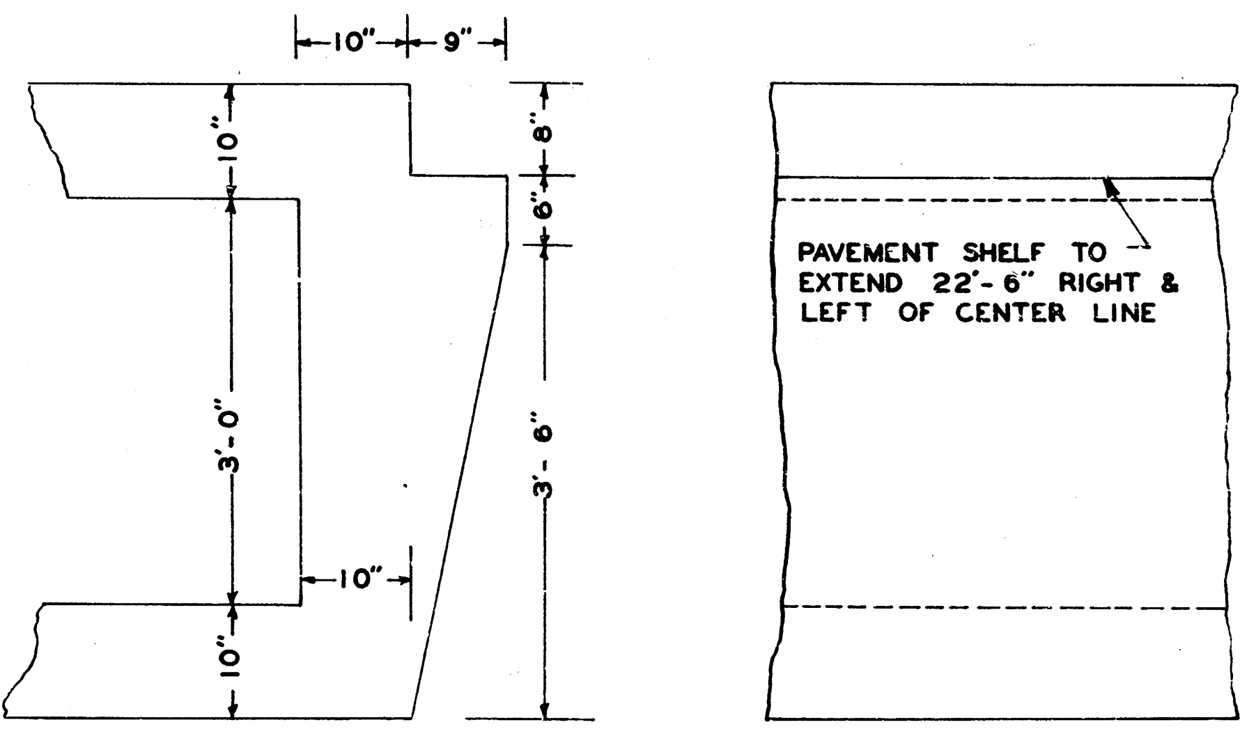
DETAIL OF PAVEMENT SHELF SCALE 1" = 1' - 0"
