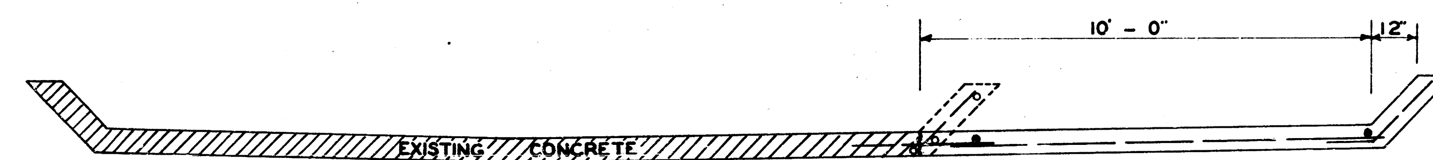
CROSS SECTION DETAIL SOUTH OF BOX CULVERT SCALE 1/2" = 1' - 0"
