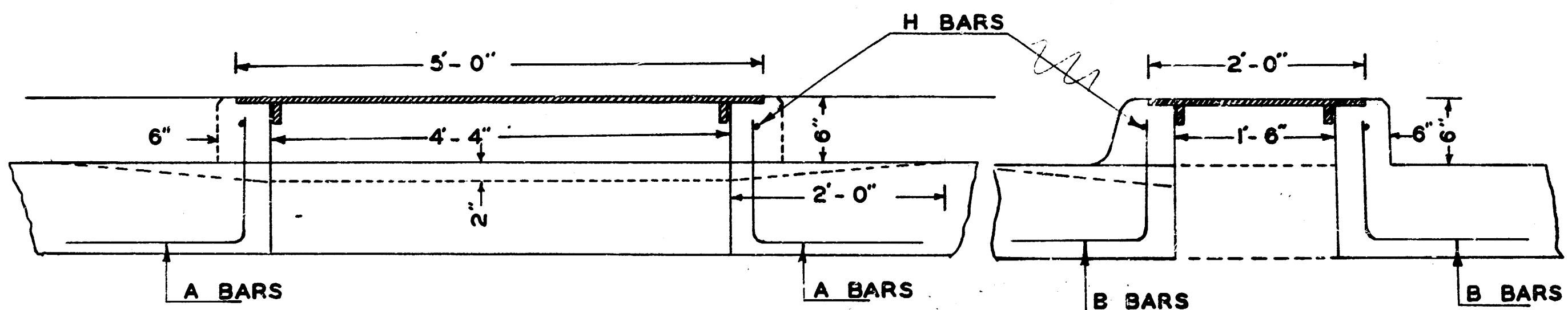
DETAIL OF CATCH BASIN SCALE 1" = 1' - 0"
