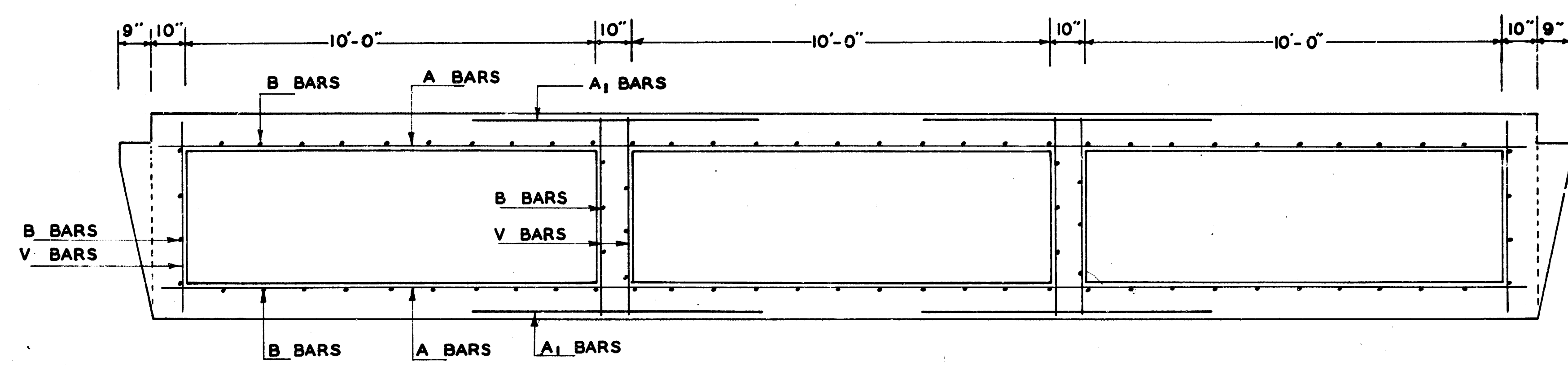
CROSS SECTION OF BOX SCALE 1/2" = 1' - 0"
