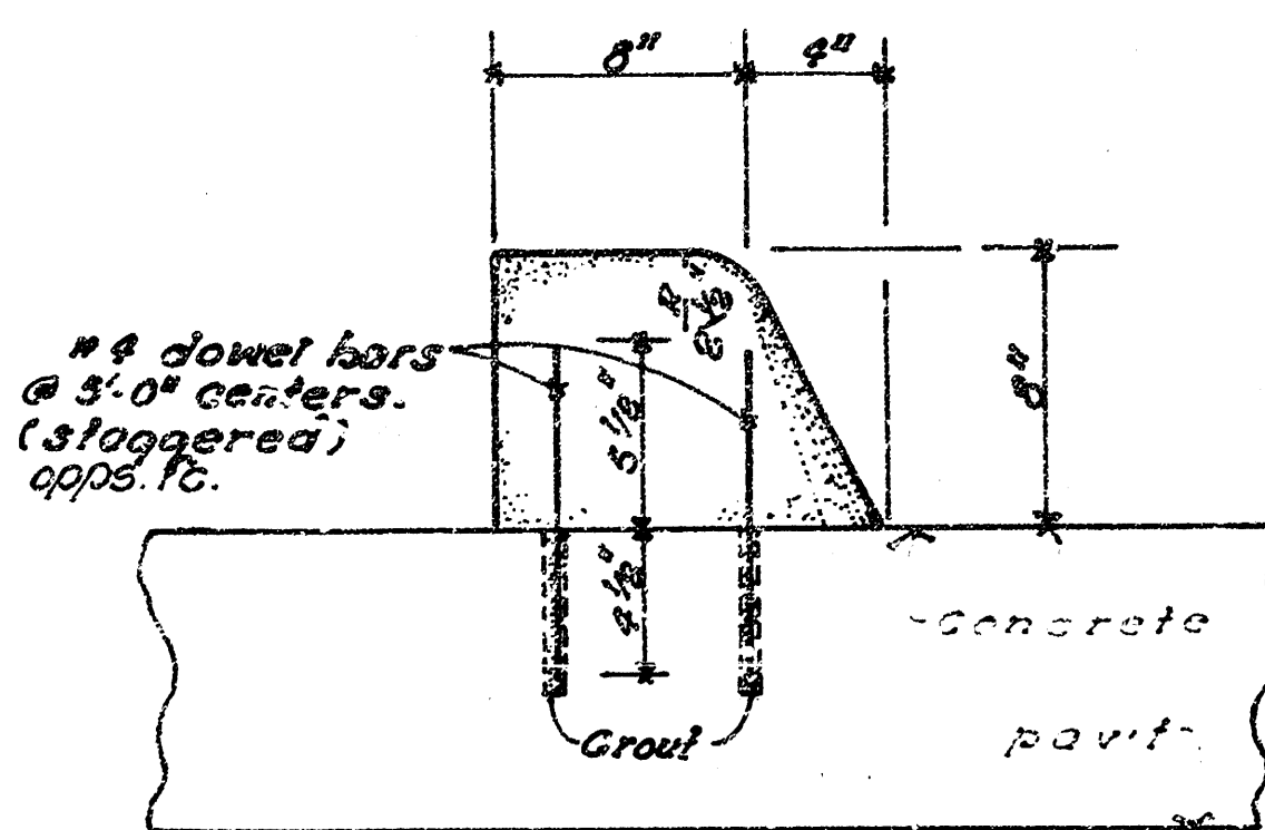
"DOMELED CURB" DETAIL (8 SOCK CONC)
