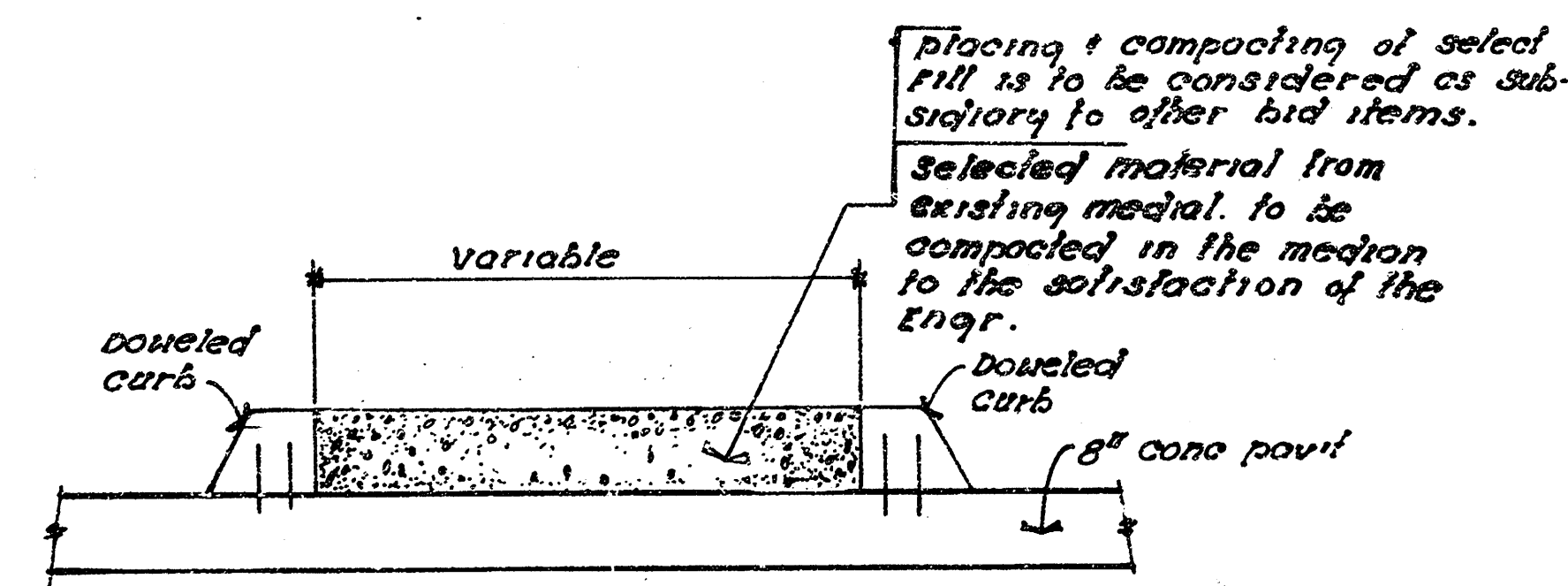
"TRAFFIC ISLAND DETAIL"
