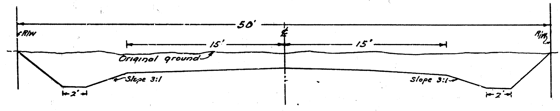
TYPICAL CROSS SECTION Scale 1"=5'
