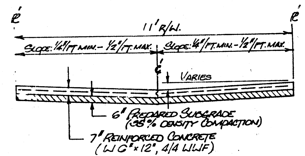
TYPICAL PAVEMENT SECTION
