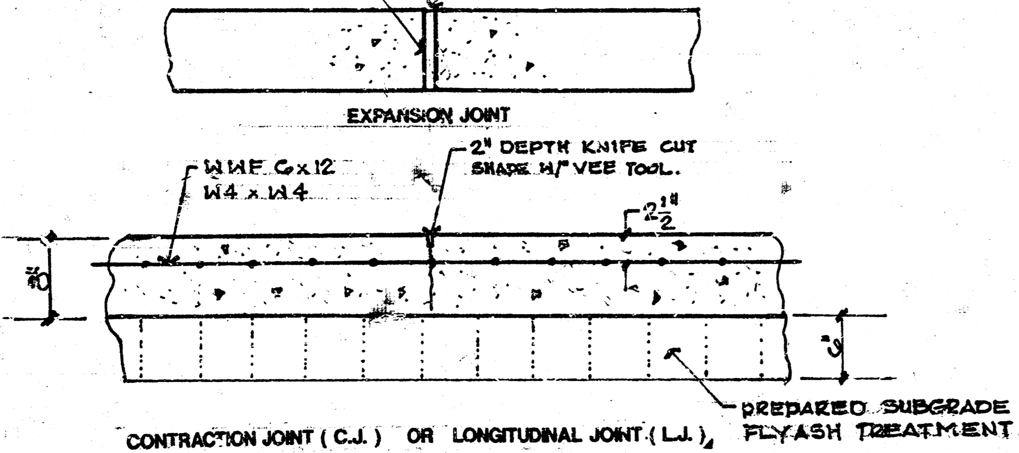
8" REINF. CONC. PAVEMENT SECTION
