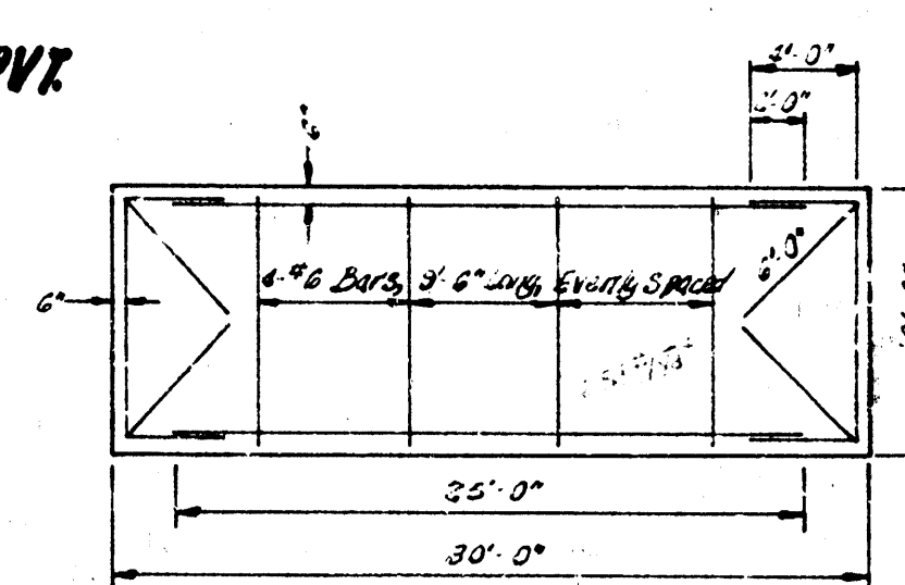
TYPICAL SECTION THRU ALLEY NOT TO SCALE
