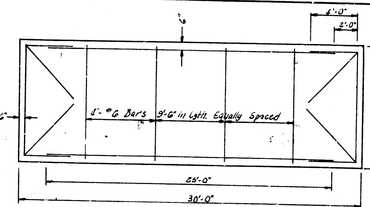
STEEL PATTERN NOT TO SCALE
