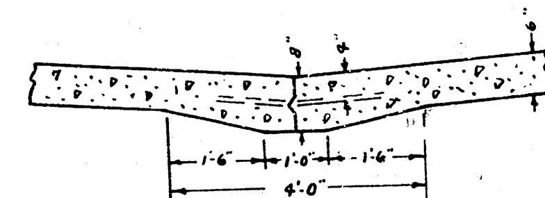
DETAIL OF MASTIC KEY JOINT No Scale
