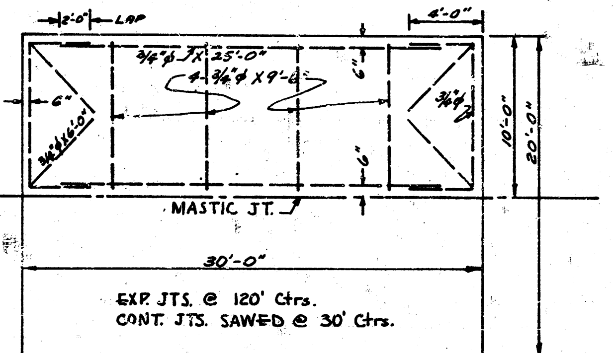
STEEL PATTERN NO SCALE
