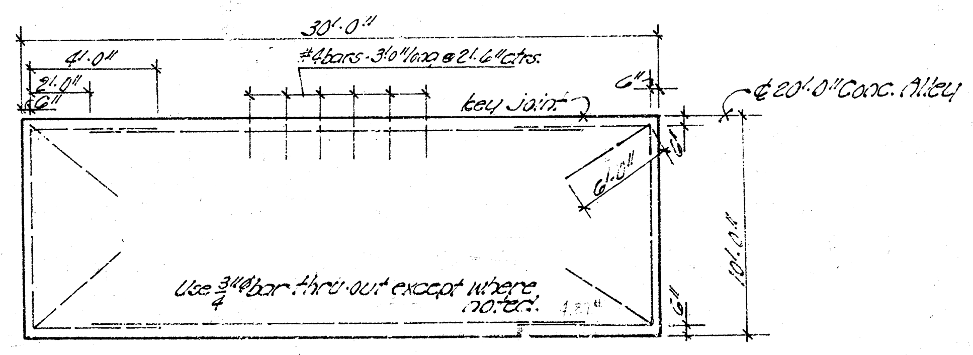
TYPICAL STEEL PATTERN (no scale)
