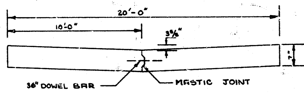
TYPICAL SECTION NO SCALE
