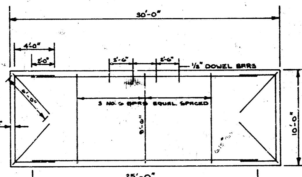
STEEL PATTERN NO SCALE
