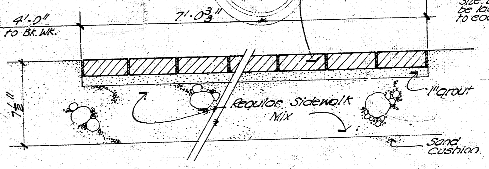
B TYPICAL SECTION 3" = 11'-0"
