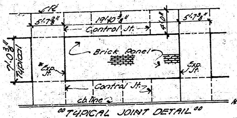
TYPICAL JOINT DETAIL Expansion Jt. Use 2" precast exp. jt.
