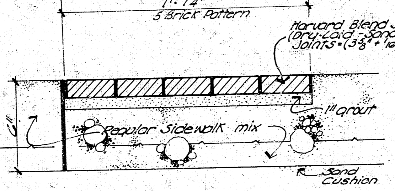
A TYPICAL SECTION 3" = 11'-0"
