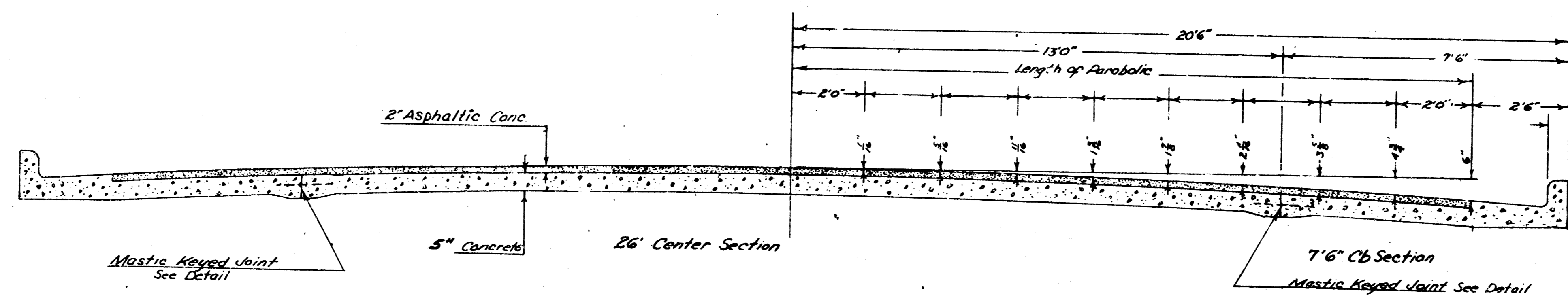
TYPICAL SECTION
