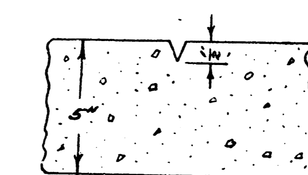
Detail Plane of Weakness Plane of Weakness to be cut with double-flve groove to depth as shown in a straight line from curb to curb 26' ctr. to ctr.
