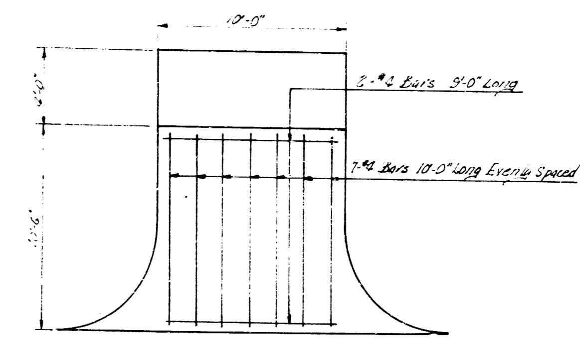
STEEL REINF. FOR DRIVES EAST SIDE ELIZABETH NOT TO SCALE
