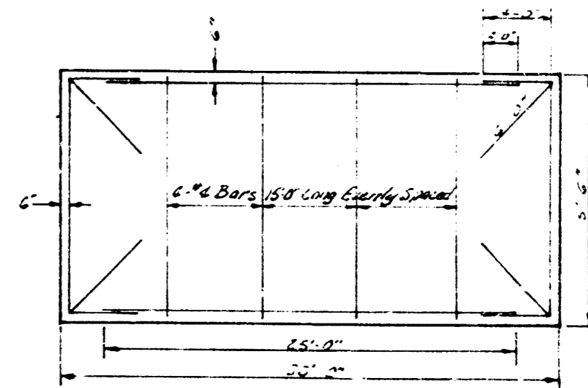
STEEL PATTERN FOR PVT NOT TO SCALE
