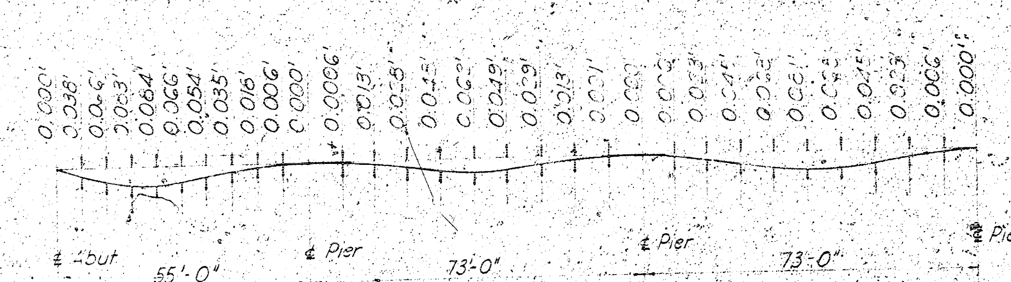
DEAD LOAD DEFLECTIONS AT TENTH POINTS
