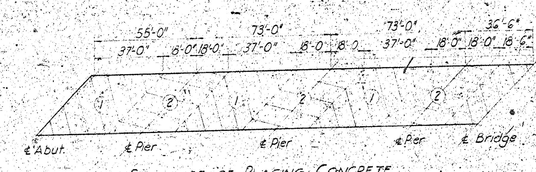
SEQUENCE OF PLACING CONCRETE
