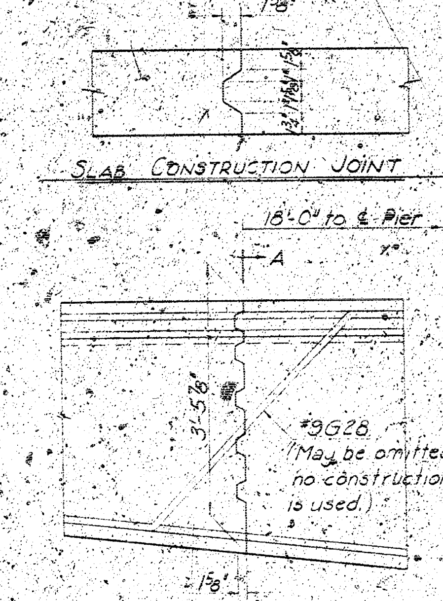
TYPICAL GIRDER CONSTRUCTION JOINT
