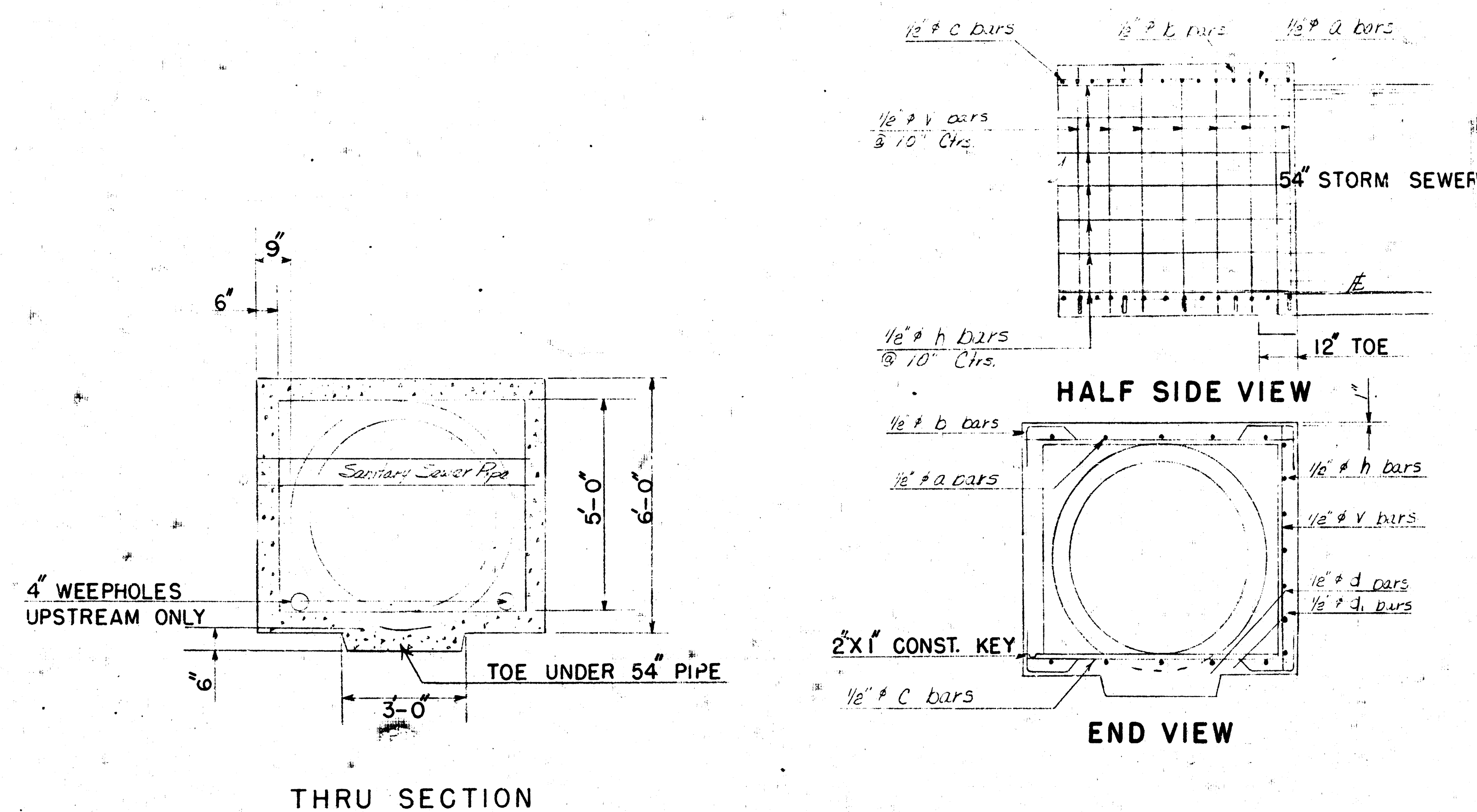
REINFORCING DETAILS
