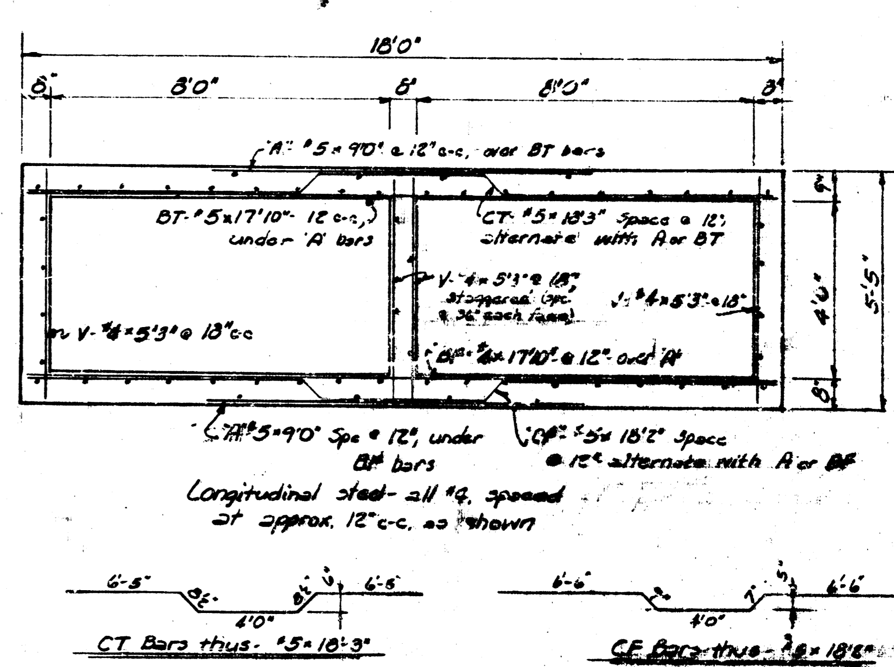
DETAILS OF TYPICAL BOX SECTION
