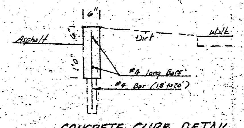
CONCRETE CURB DETAIL
