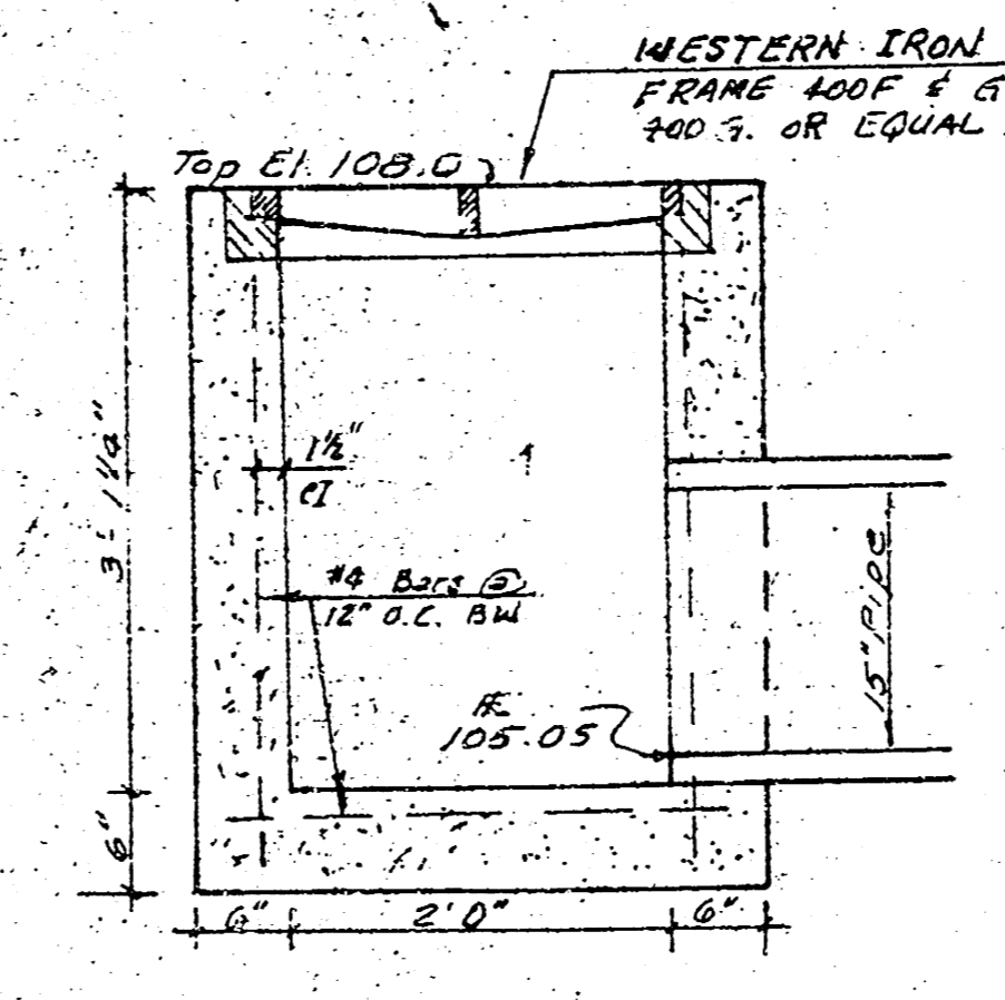
DROP INLET DETAILS 3/4" x 1"
