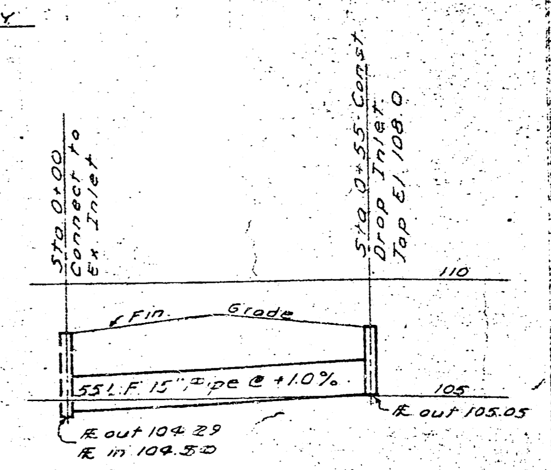
STORM SEWER PROFILE
