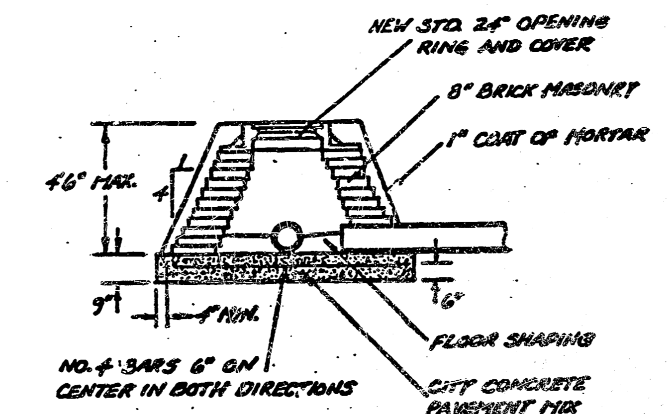
SHALLOW SPECIAL MANHOLE "TYPE A"
