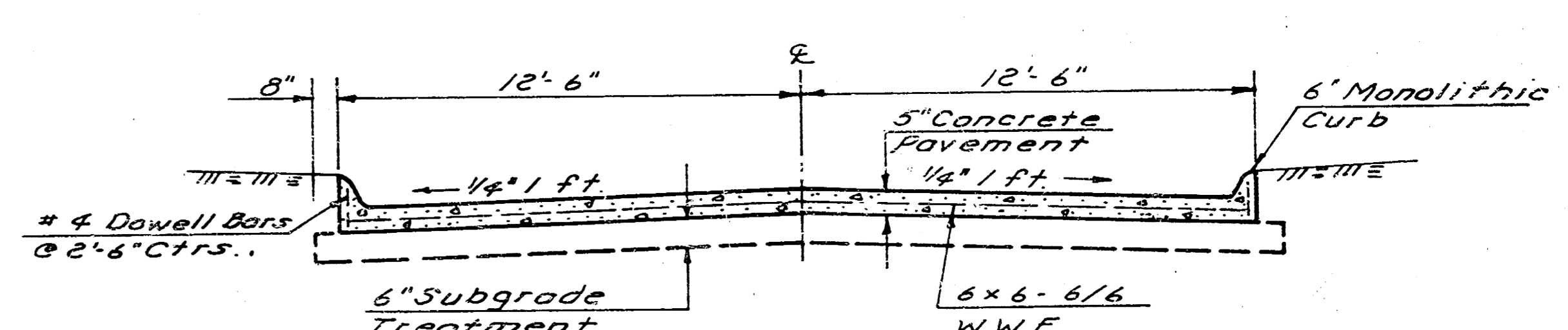
TYPICAL SECTION - 25'-B-B PAVEMENT
