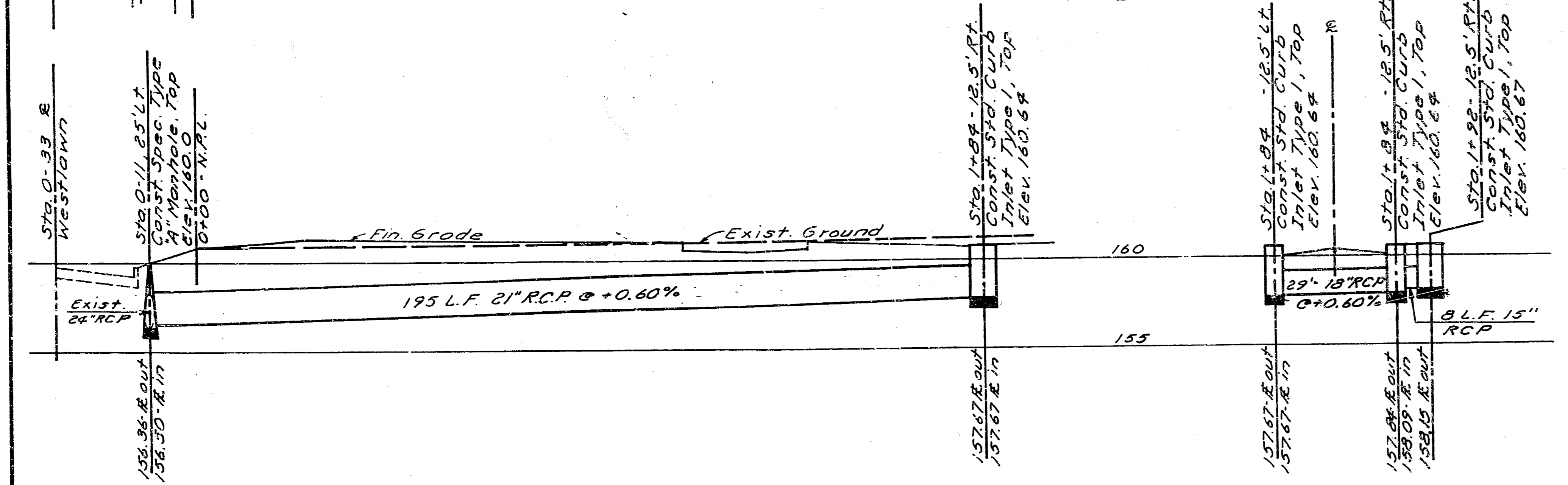
STORM SEWER PROFILES
