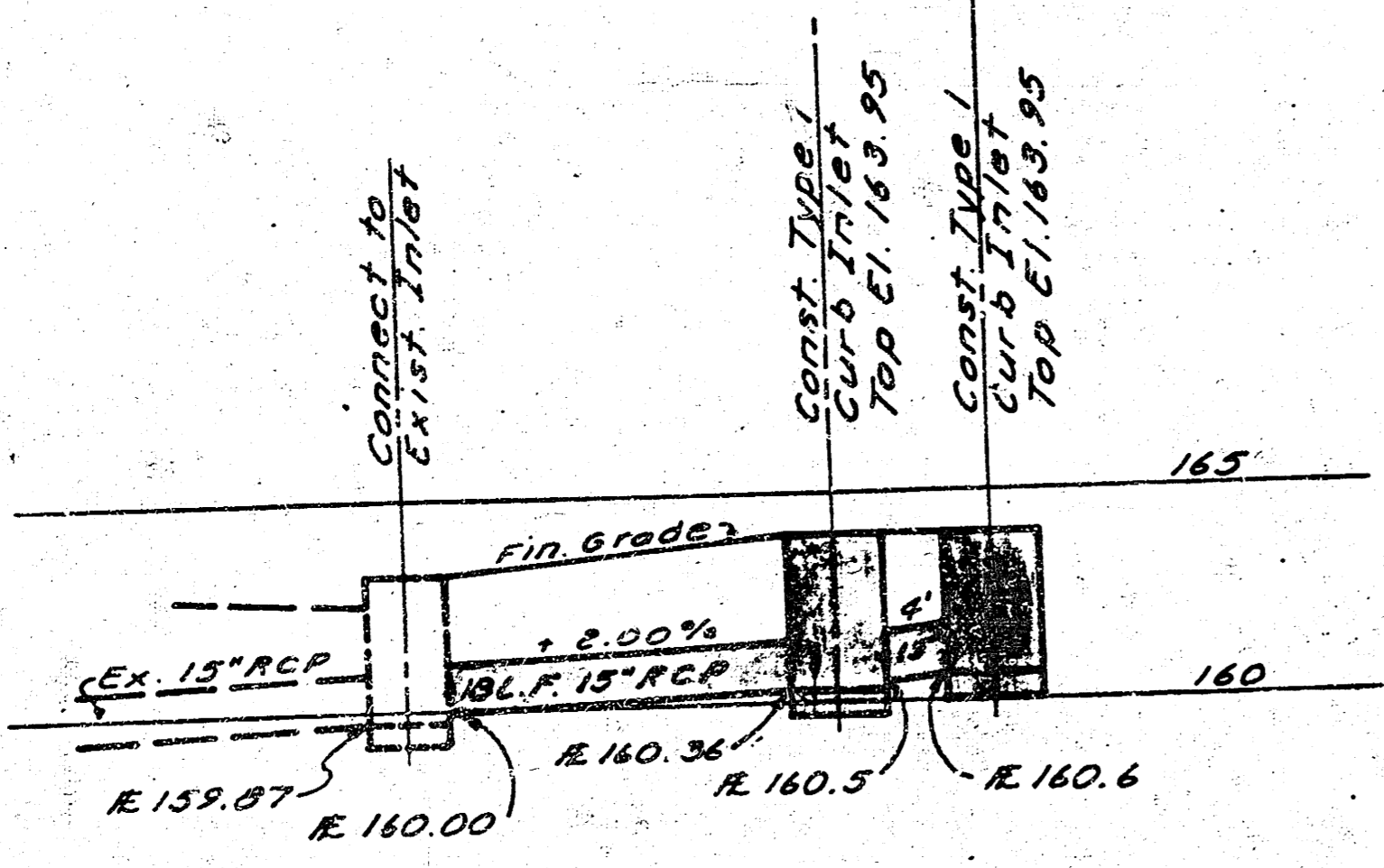
STORM SEWER PROFILE Scale: Hor. 1" = 10' Ver. 1" = 5'
