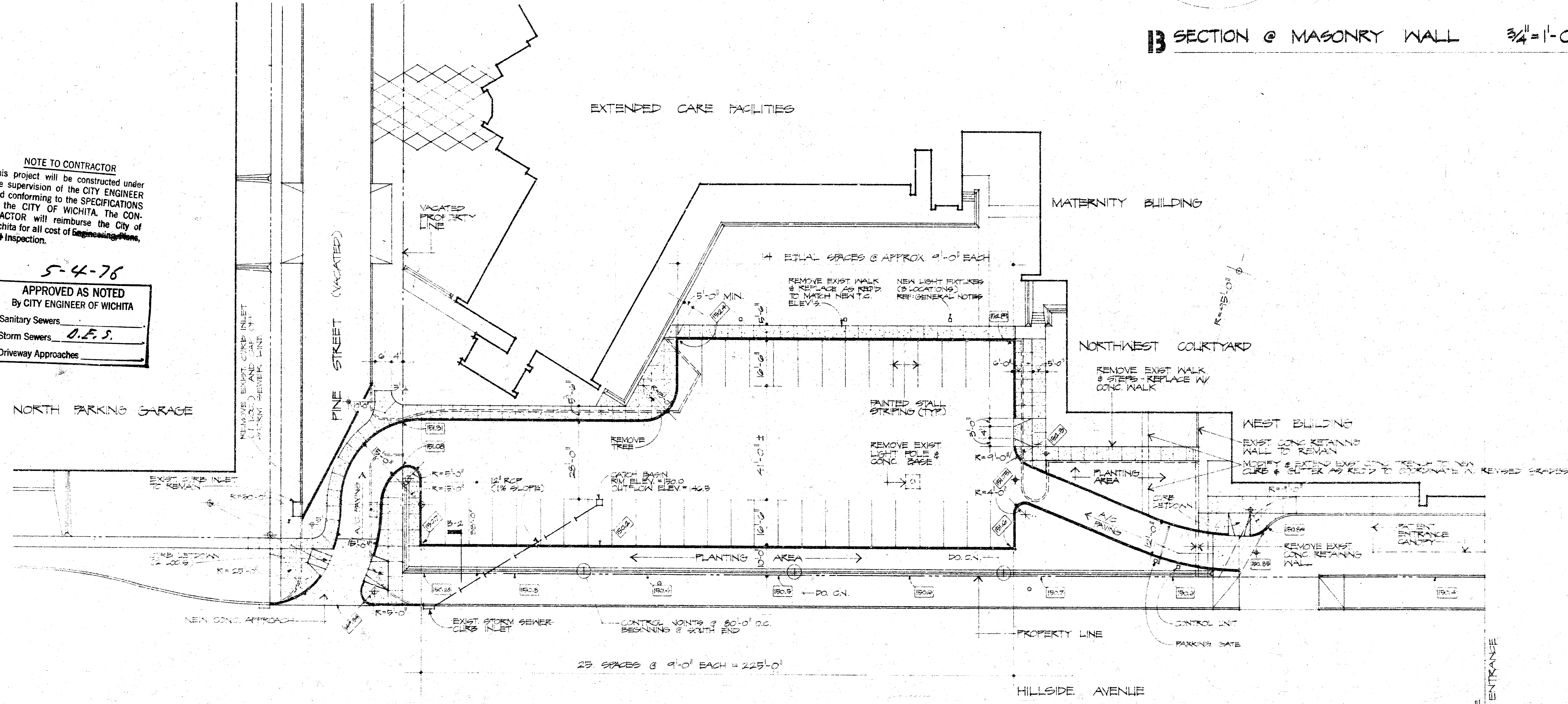
1" = 20' SITE PLAN/PARKING LOT "C"
