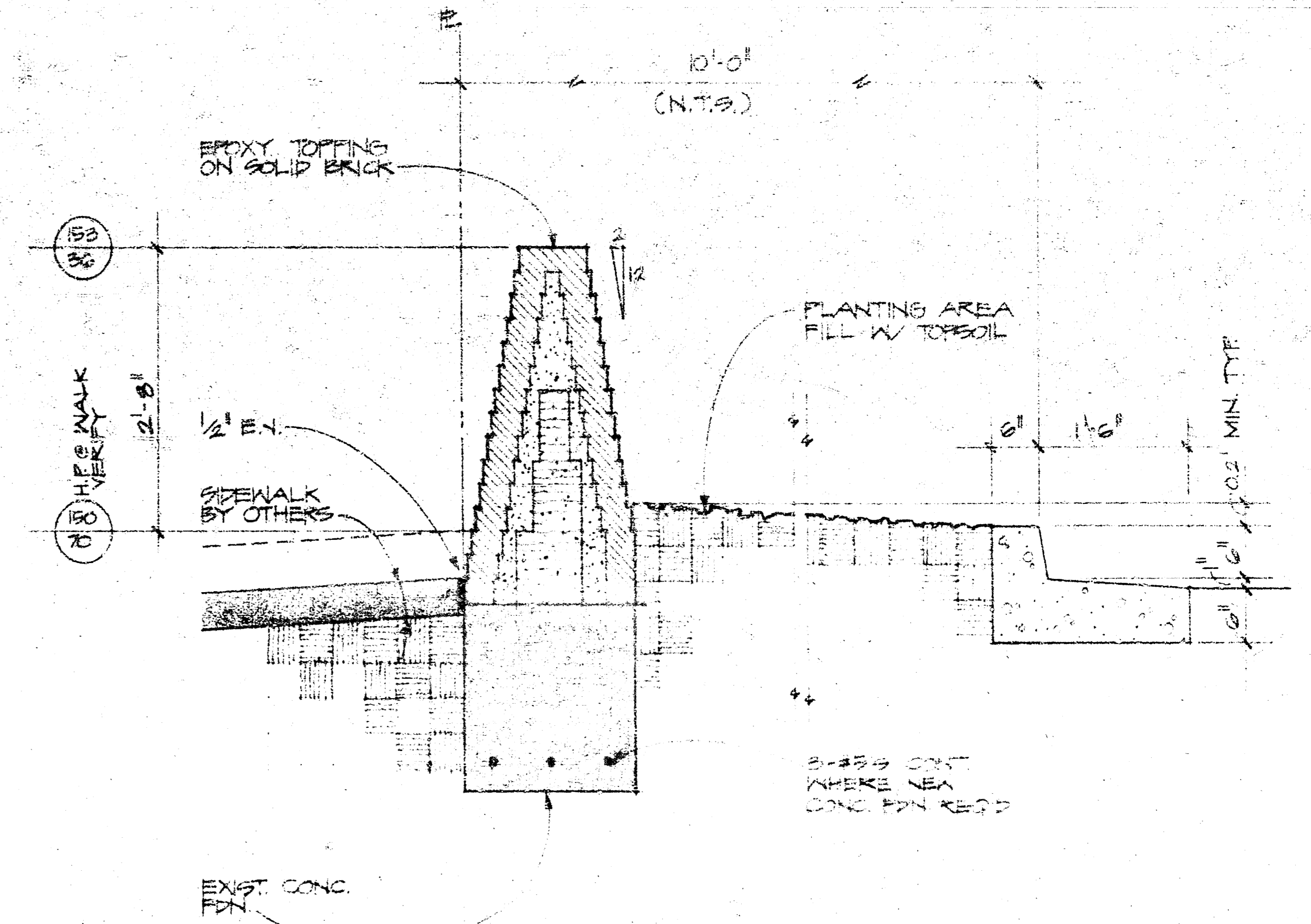
SECTION @ MASONRY WALL 3/4" = 1'-0"
