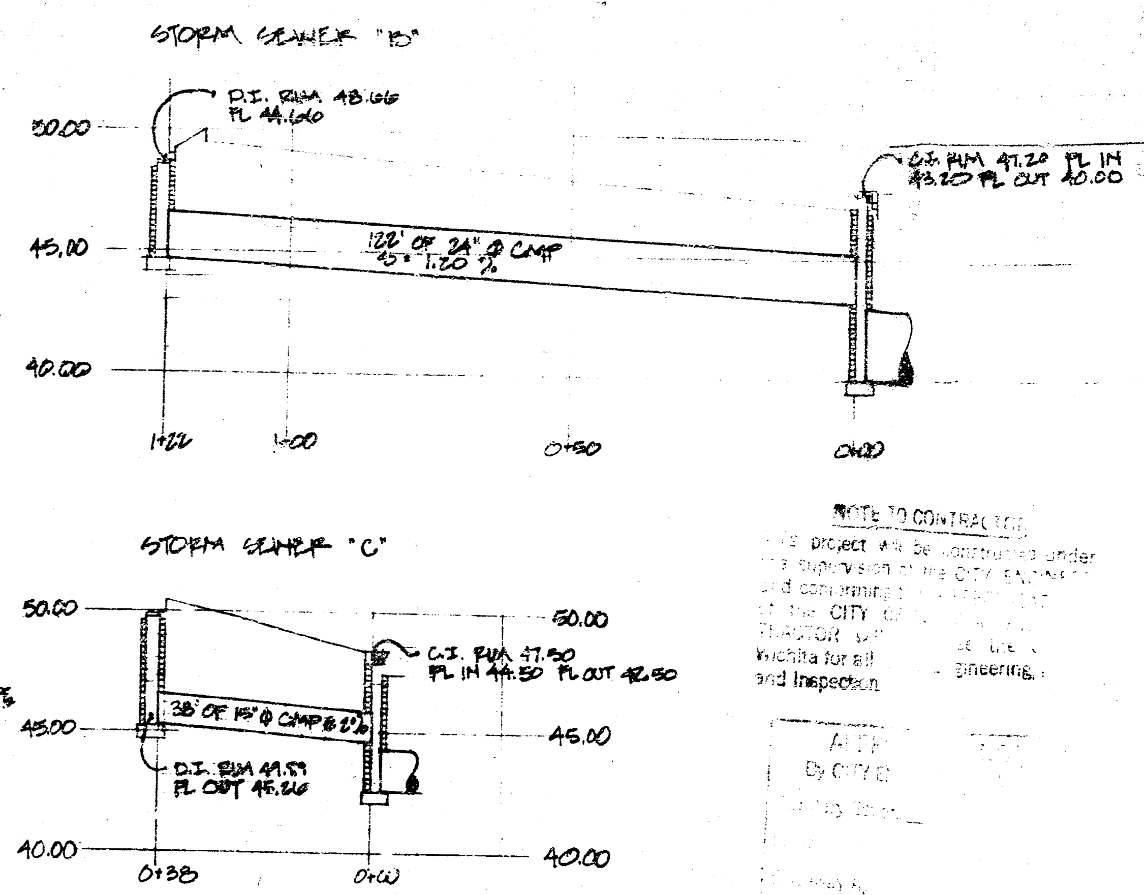
1 PRIVATE STORM SEWER PROFILES HORIZONTAL SCALE 1"=20' VERTICAL SCALE 1"=5' CITY OF WICHITA PRIVATE STORM SEWER PROJECT NO. 468-710-245-80847
