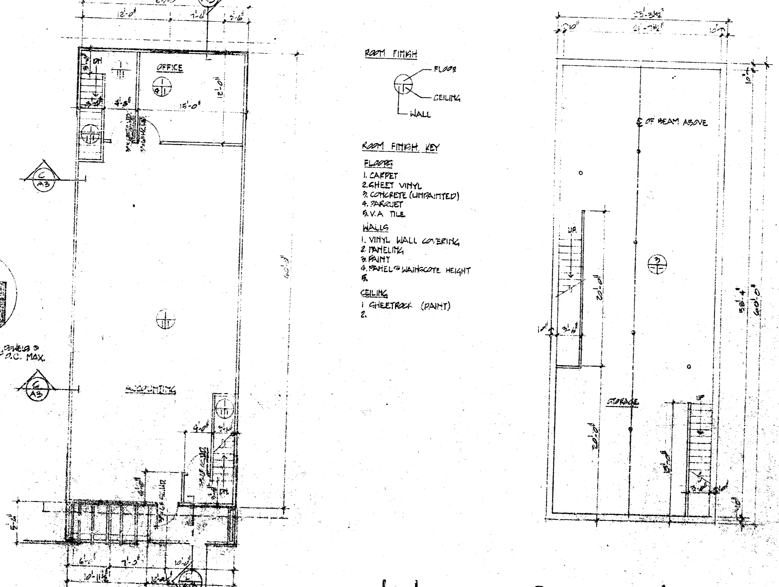
FLOOR PLAN
