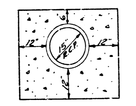
ENCASEMENT DETAIL 6-INCH CONCRETE
