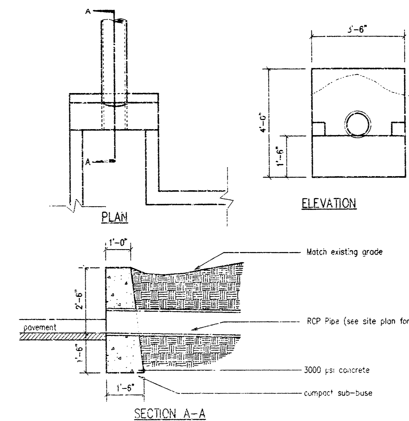
1 CONCRETE HEADWALL Scale: 3/8" = 1'-0" C_HEADWALL
