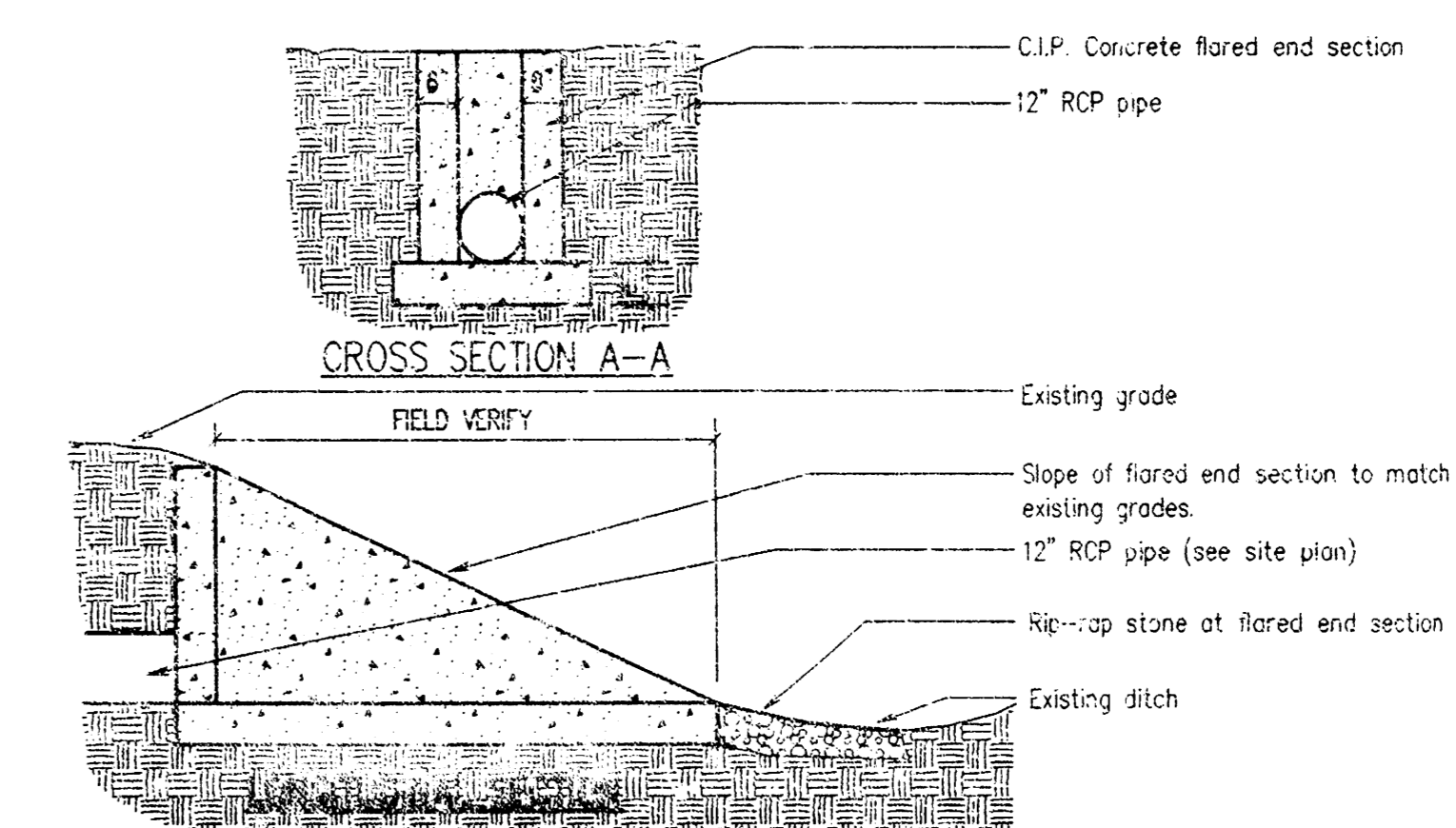
2 CONCRETE FLARED END SECTION IN ROW Scale: 3/8" = 1'-0" C_CONCEND
