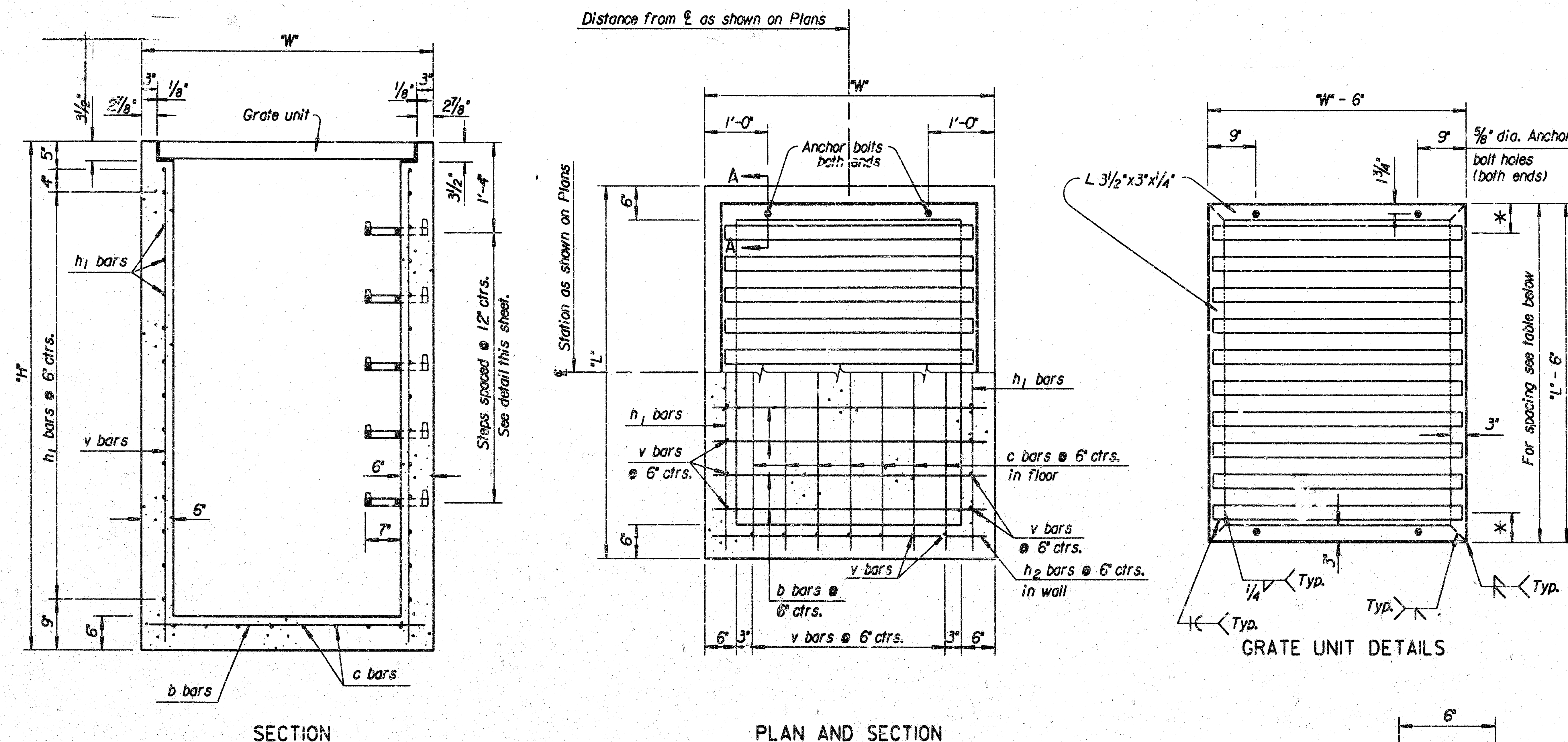
SECTION
