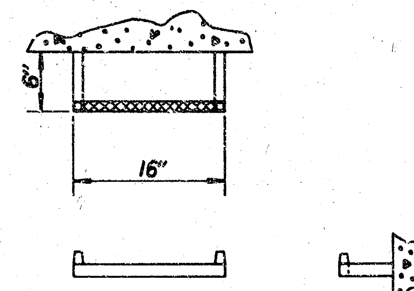
STEP DETAILS
