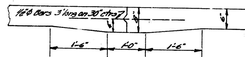
Mastic Joint Detail No Scale
