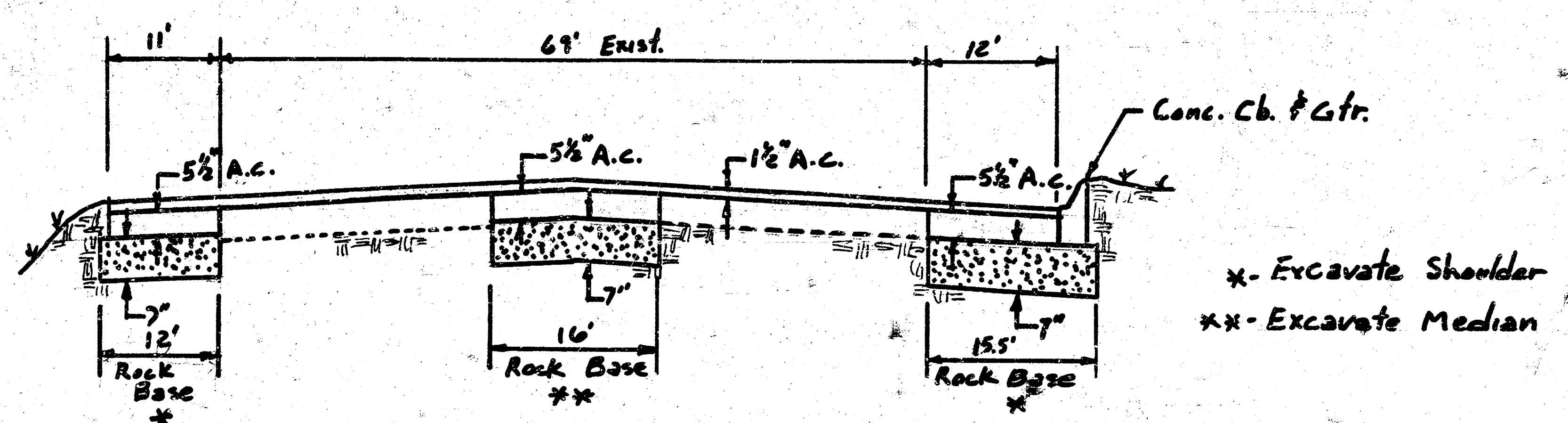
SECTION B-B
