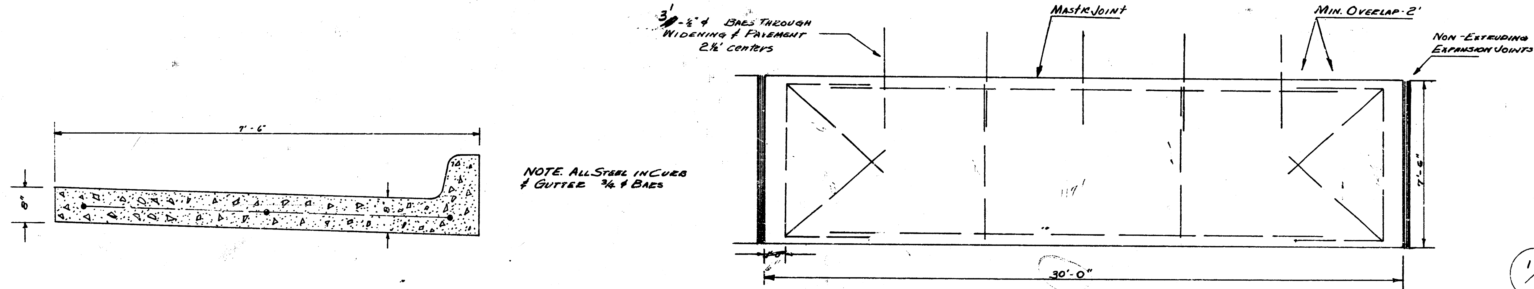
DETAILS OF CURB & GUTTER
