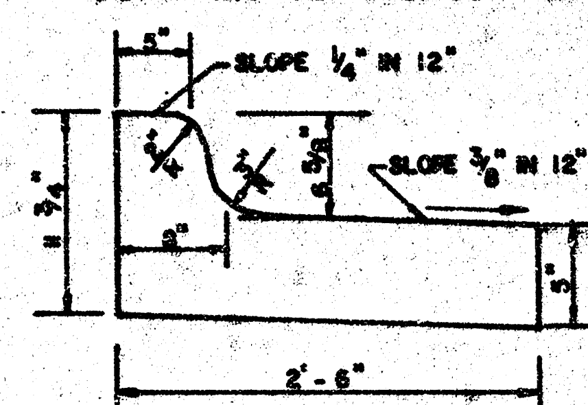
COMBINED CURB & GUTTER (MEDIAL)
