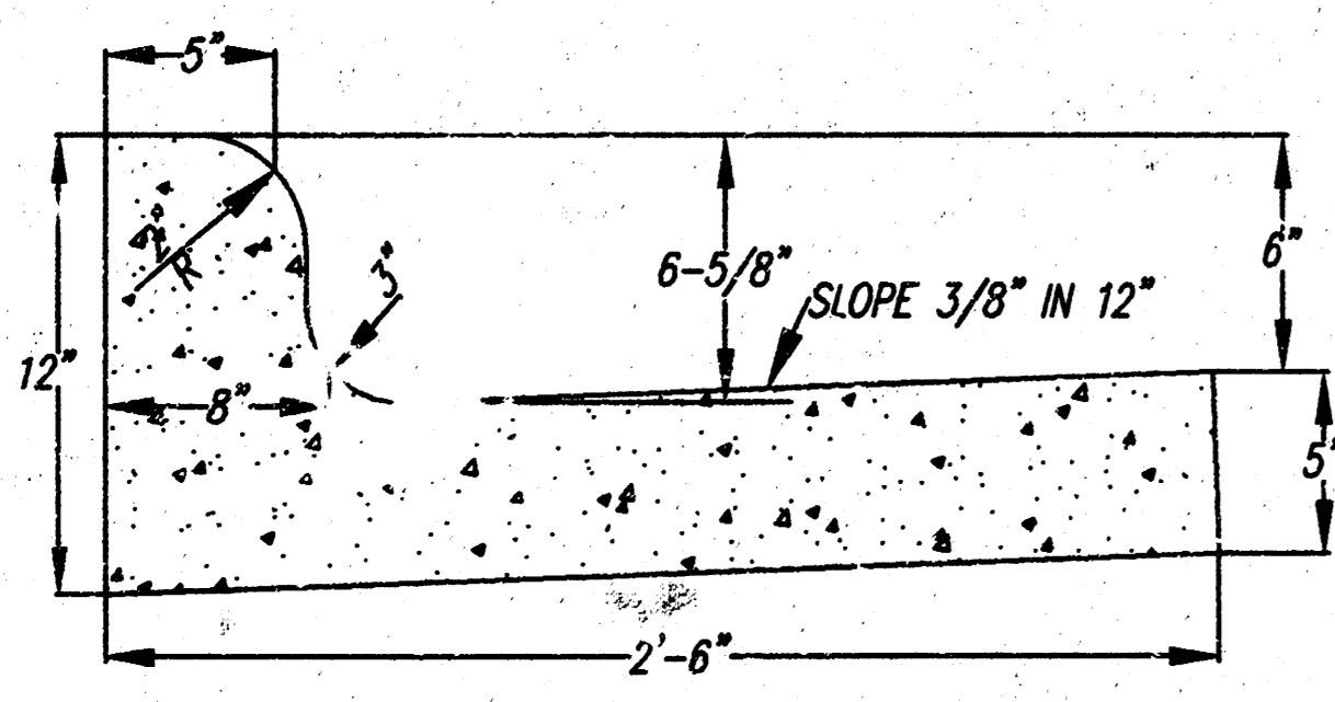
COMBINED CURB & GUTTER
