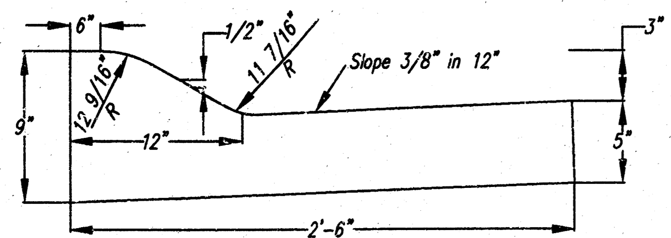
ROLL TYPE COMBINED CURB & GUTTER
