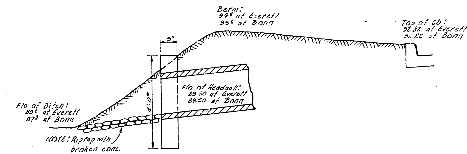
SECTION THRU BANK AT HEADWALL NOT TO SCALE
