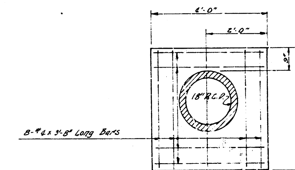
ELEV OF REINFORCED CONCRETE HEADWALL NOT TO SCALE
