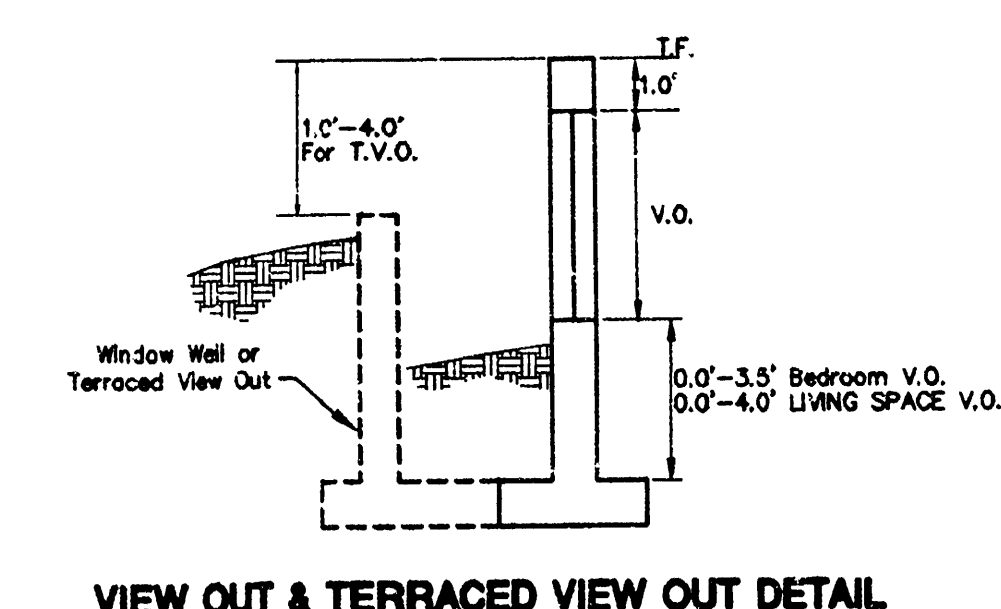
VIEW OUT & TERRACED VIEW OUT DETAIL
