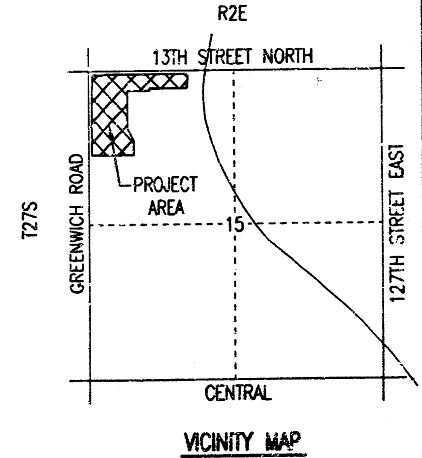
VICINITY MAP
