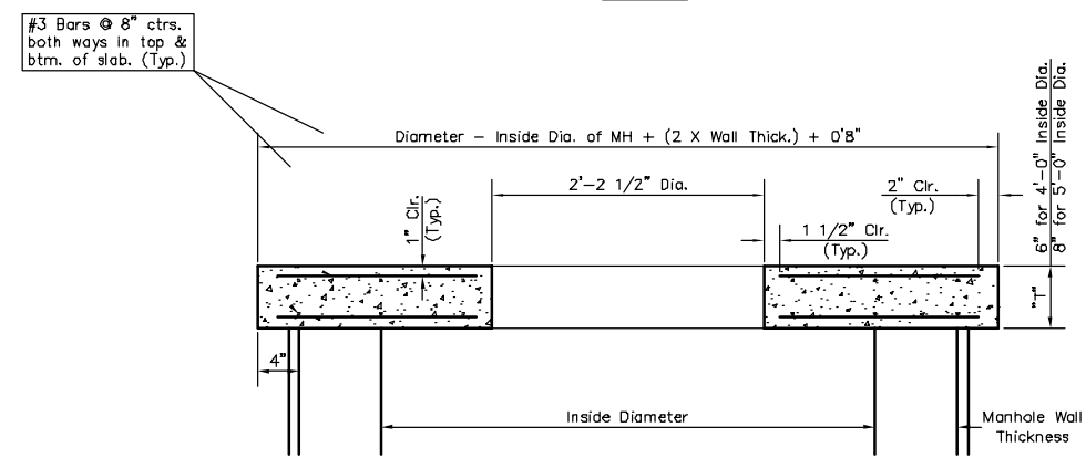
SECTION A-A CONCRETE SLAB DETAILS
