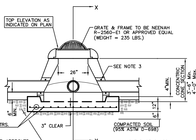
SPECIAL SHALLOW TYPE "P" MANHOLE WITH BEEHIVE FRAME & GRATE
