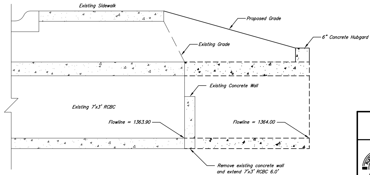
BOX CULVERT DETAIL
