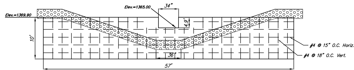
WEIR DETAIL
