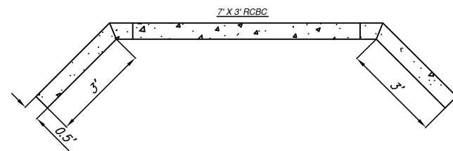
BOX AND WING WALL DETAIL (TOP VIEW)
