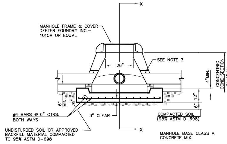
SPECIAL SHALLOW TYPE "P" MANHOLE
